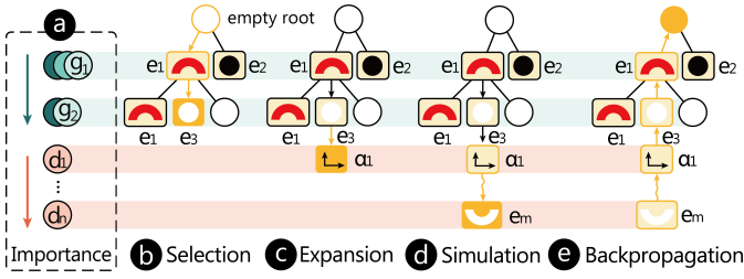
Fig. 4. (a) The data dimensions and groups are ordered by importance independently. An iteration of the Monte Carlo tree search consists of four stages, including (b) selection, (c) expansion, (d) simulation, and (e) backpropagation. The shapes with a yellow frame represent the operation of this stage. Inside the nodes are element thumbnails ( e_i ) or axes ( \alpha_i ). Circles with no elements are empty nodes ( \emptyset ).
