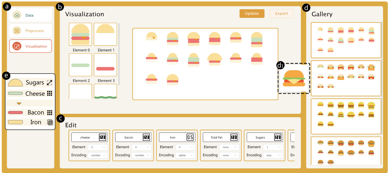
Fig. 5. The interface of MetaGlyph is consisted of : (a) a Menu view for different steps; (b) an MGv view representing visual elements and corresponding MGv, (c) an Edit view, in which the data mappings can be modified based on user's preferences, and (d) a Gallery view with other MGv options. (e) concrete data mappings for the MGv view in detail.
