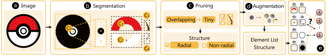
Fig. 3. The entire process of metaphoric image selection for each (a) input online image, including (b) segmentation: dividing the image into visual elements, (c) pruning: deleting redundant elements and determining the structure, and (d) augmentation: checking if some elements can transform into charts. The output is an element list with an image structure. (e) The mapping space for constructing MGVs.
